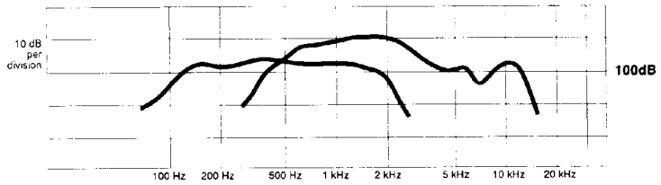
DTH1 Low: High Band Curves Bi-Amp Mode: User must set crossover for mid to high point
